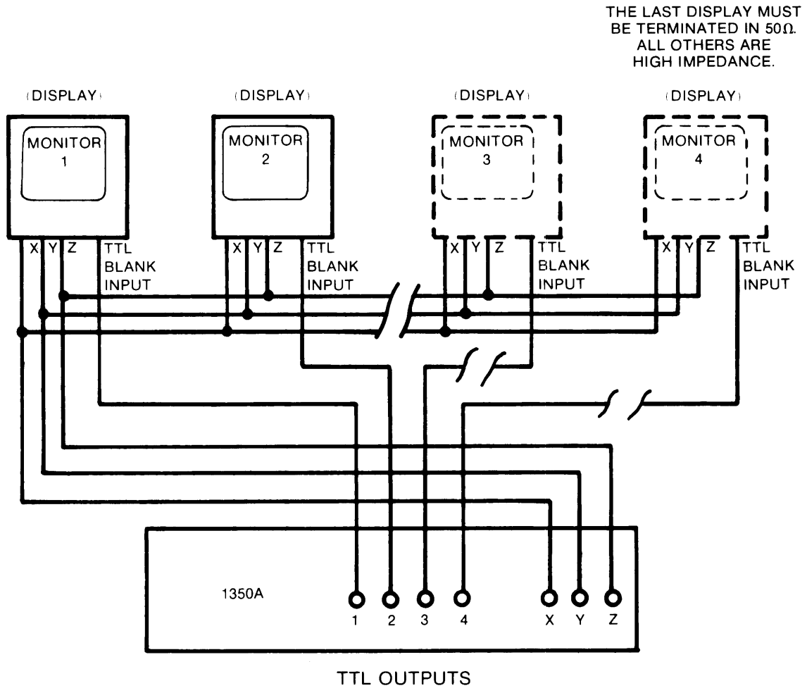
Figure 5-1. 1350A/Display Interconnections
